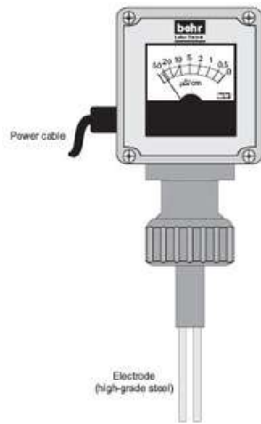
LFD Conductivity meter
